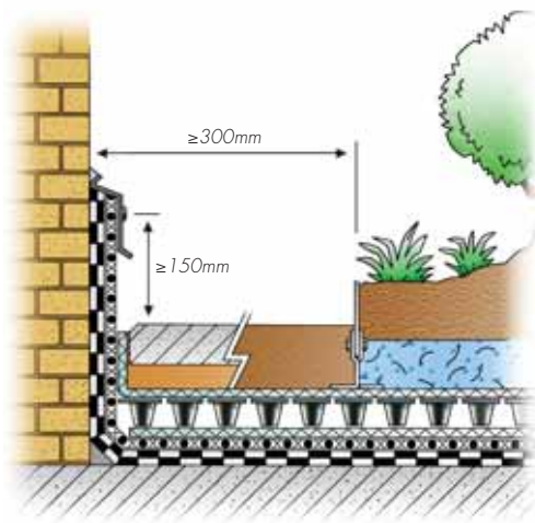
Detail 2. Facade
