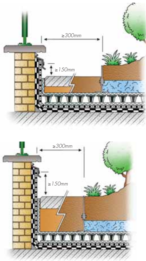
Detail 1. Parapet
